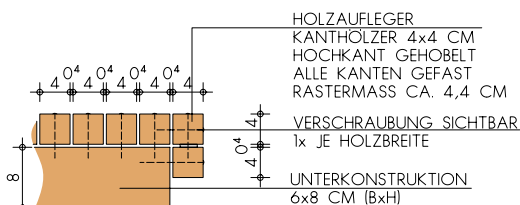
DETAIL: BLENDHOLZ 1:5
